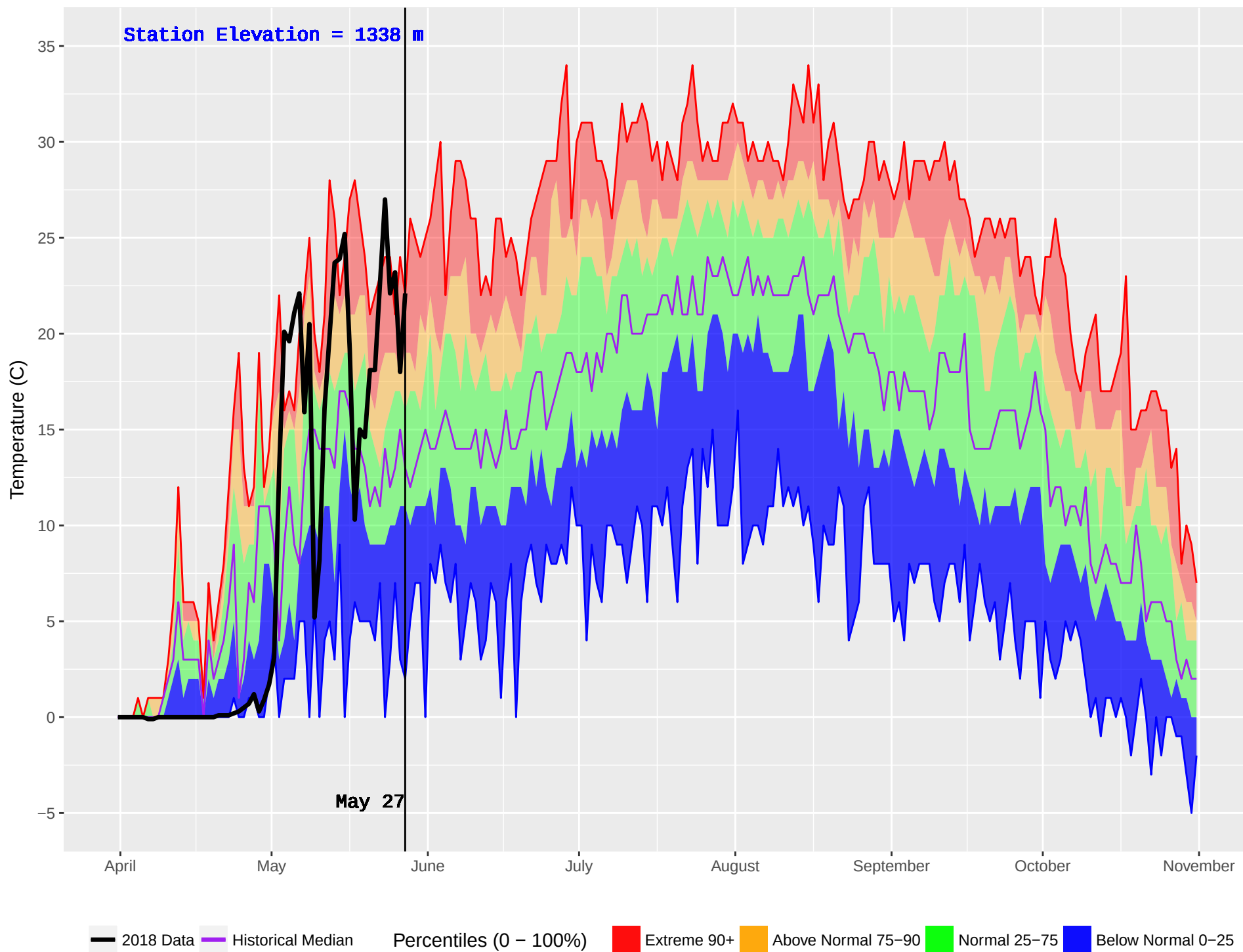
EIGHT MILE (391) : Historical (1980–2016) and Current (2018) Noon Temperature
