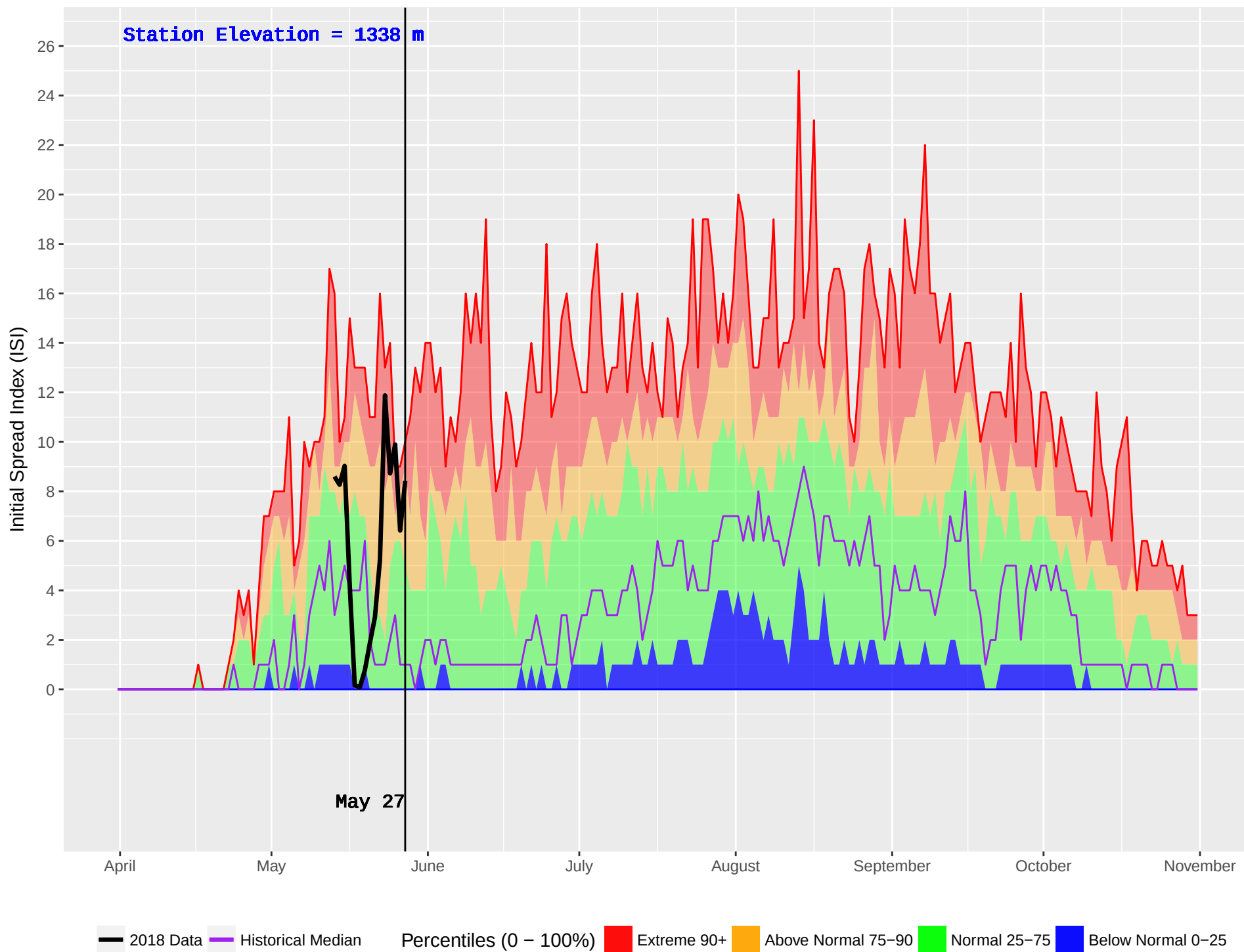
EIGHT MILE (391) : Historical (1980–2016) and Current (2018) Noon Initial Spread Index (ISI)
